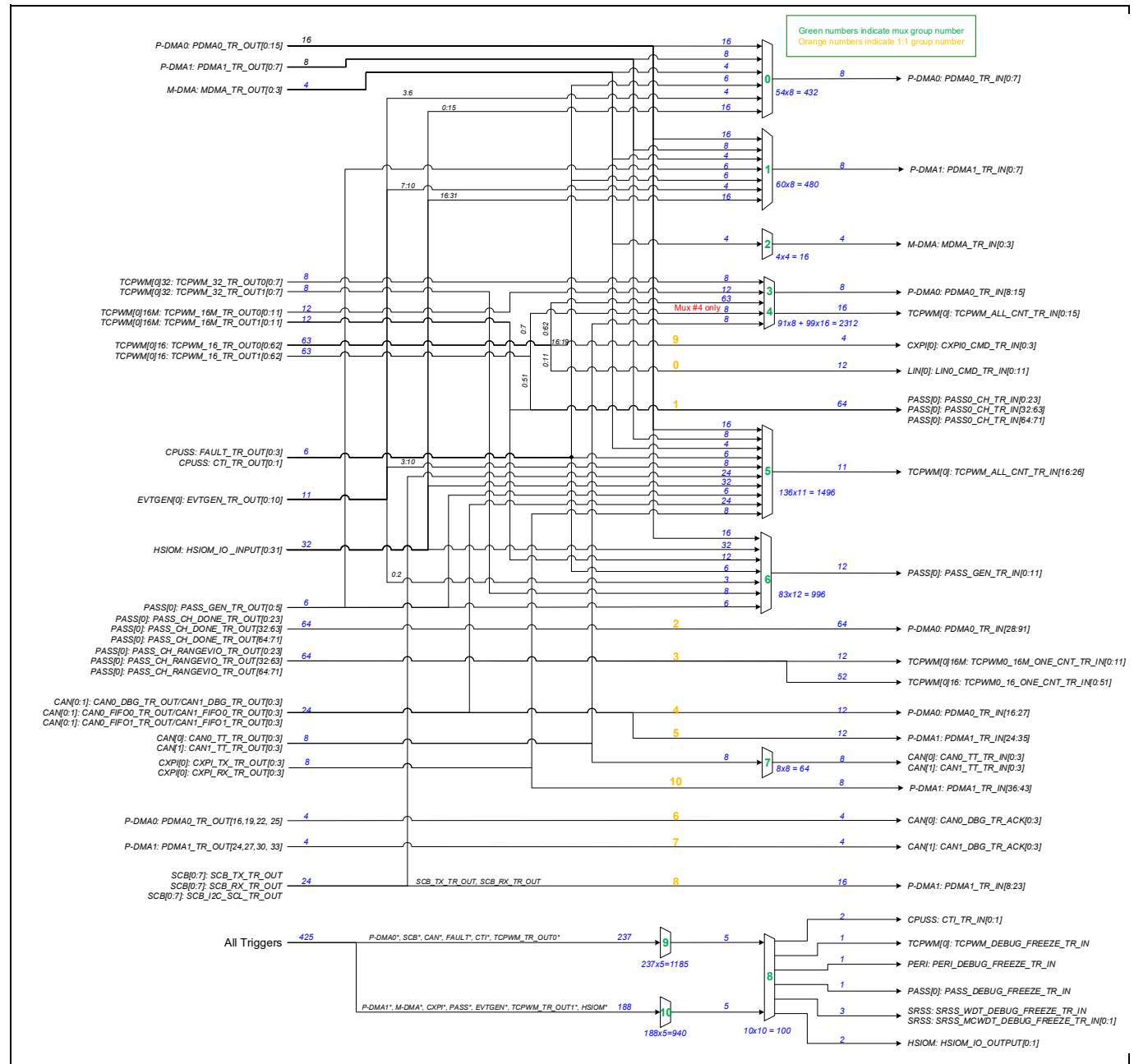
Figure 16-1 Trigger multiplexer [31]
