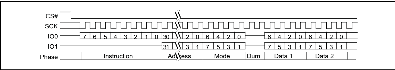
Figure 80 Dual I/O read command sequence (4-byte address, BCh or BBh [ExtAdd = 1], EHPLC = 10b)
