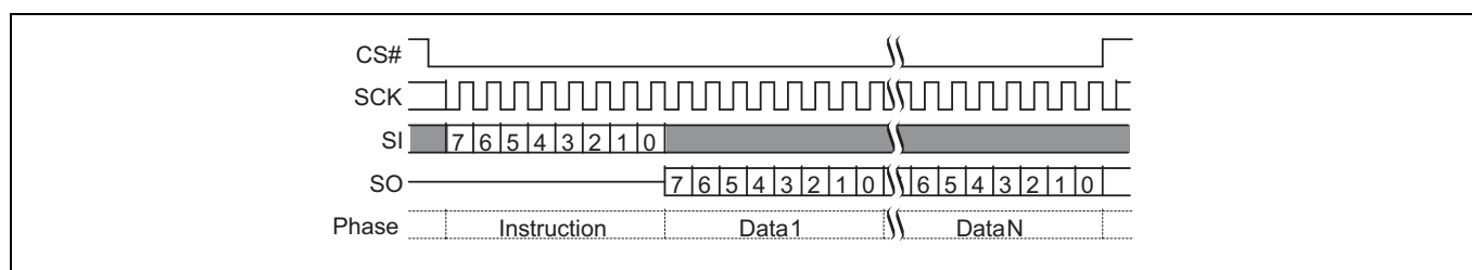
Figure 65 AutoBoot register read (ABRD 14h) command
